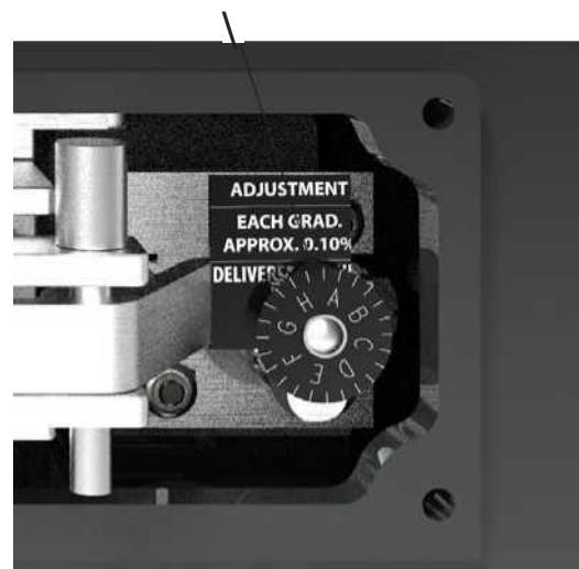
Calibration Adjustment Screw
